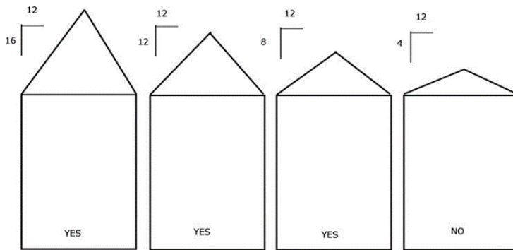
Roof Pitch Examples (Drawing Not To Scale)
