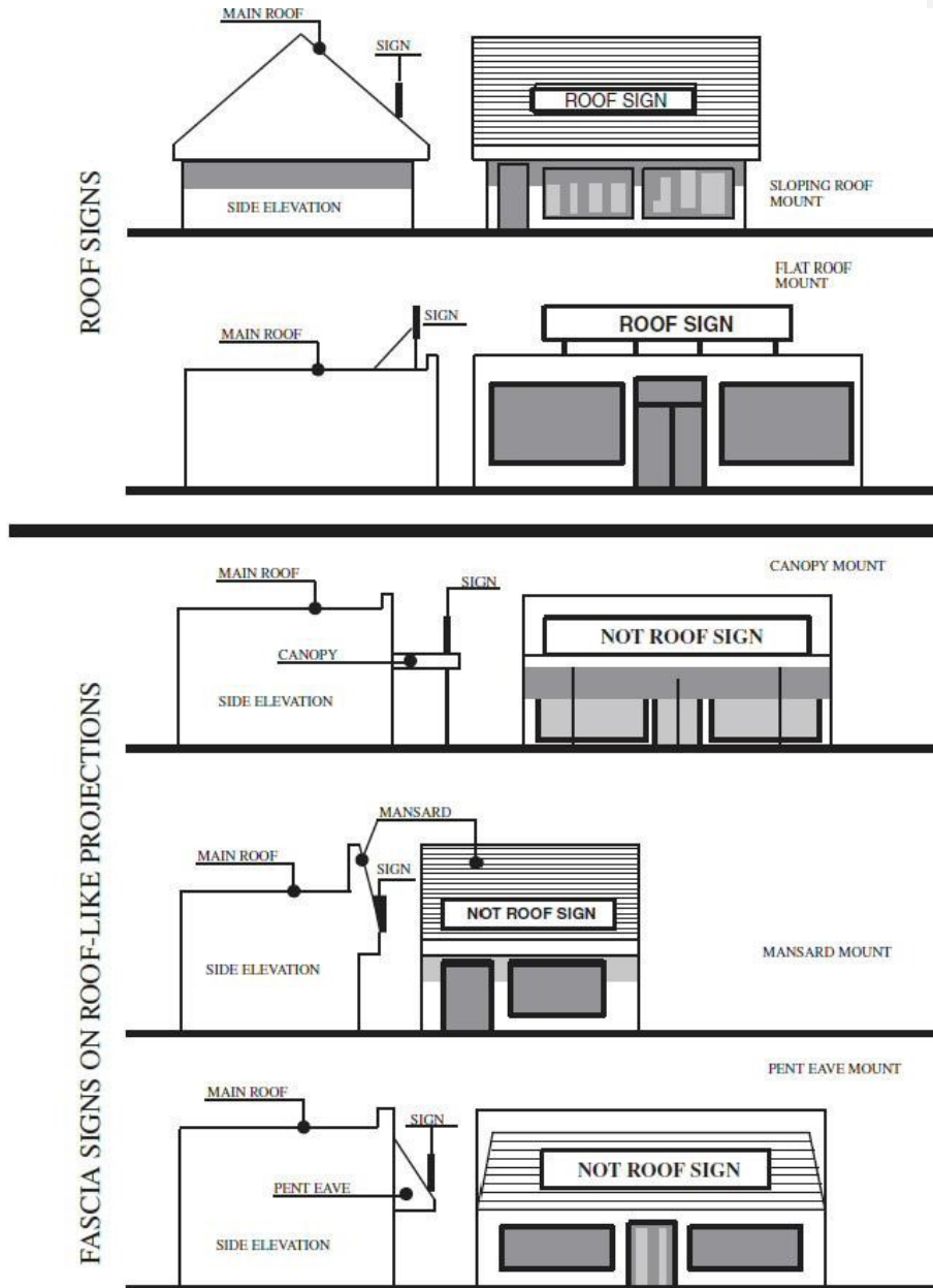
FIGURE C.1(2) COMPARISON—ROOF AND WALL OR FASCIA SIGNS
