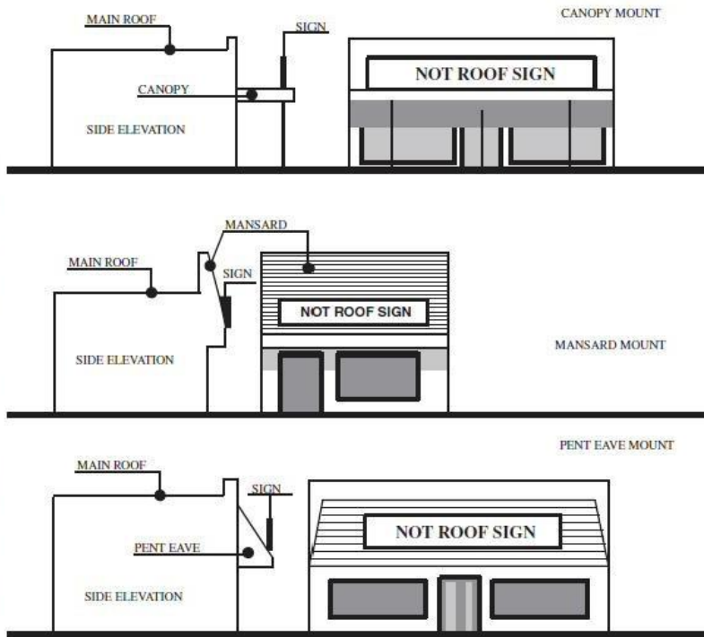
FIGURE C.1(2) COMPARISON—ROOF AND WALL OR FASCIA SIGNS
